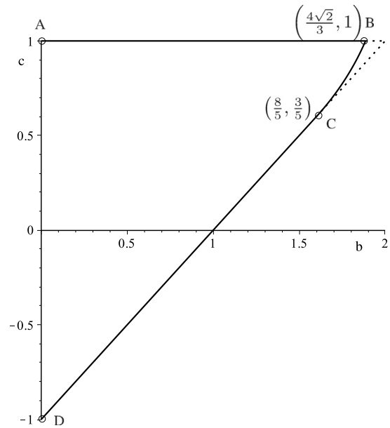
Fig. 20. The region over which the mapping (101) remains univalent for b > 0 . Between B and C, the curve is b^2/4 + 4(c/3 - 1/2)^2 = 1 . Between A and B, there are two cusps f' = 0 at \xi = -b/2 \pm i\sqrt{4 - b^2}/2 , between C and D there is a single cusp f'(-1) = 0 . Between B and C, two sides of the interface touch to enclose a bubble.
