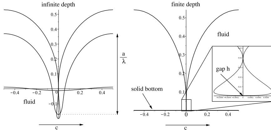
Fig. 22. Waves traveling at speed c on a quiescent fluid, as described by (121). On the left, the fluid is of infinite depth for B = 4, 1 , and B = B_c = 0.78818 \dots , while on the right, the x -axis is a solid bottom. For infinite depth, the profile self-intersects at a critical amplitude. For finite depth, we show the profile (122), (123) for k = 0.9 and B = 0.8731 , for which a bubble is formed. In the limit k \rightarrow 1 the size of this bubble goes to zero.
