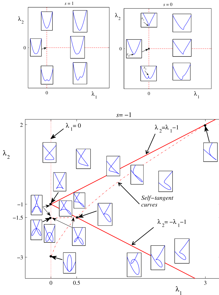
Fig. 9. Bifurcation curves for the E_6 singularity, as represented in its scaled form (43). On top, unfolding for s = 1 and s = 0 , at the bottom, the bifurcation diagram for s = -1 [9].
