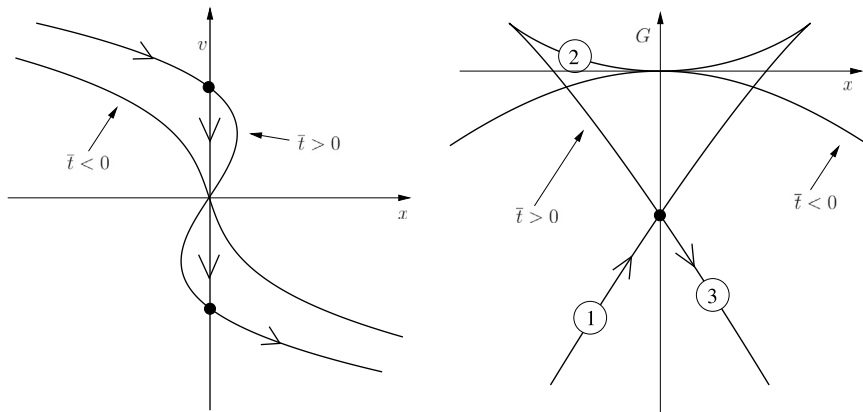
Fig. 16. Shock formation in the inviscid Burgers' equation. On the left, an initially single-valued profile develops into a three-valued s-curve. In a saddle-point approximation, the profile is constructed by moving along the potential, shown on the right. In the multi-valued region, the dominant contribution comes from the most negative value of the potential, leading to a shock position satisfying the equal-area rule.
