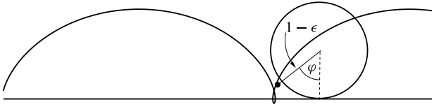
Fig. 4. A trochoid is the trajectory of a point fixed on (or external to) a rolling disk, shown here for \epsilon < 0 .
