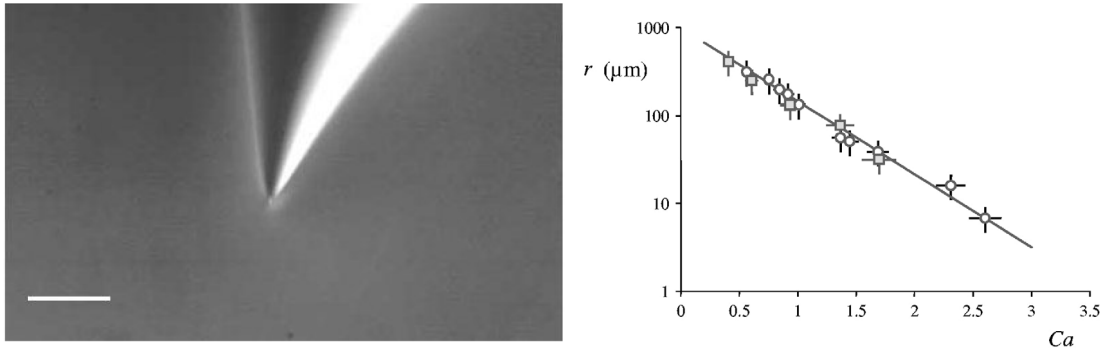
Fig. 21. Experimental data on the cusping of a viscous fluid, taken from [63]. On the left, a closeup of the tip of a cusp on the surface of a viscous fluid; the scale bar corresponds to 200 \mu\text{m} . On the right, the radius of curvature of the (almost) cusp as function of capillary number. In agreement with (113), the dependence is exponential.
