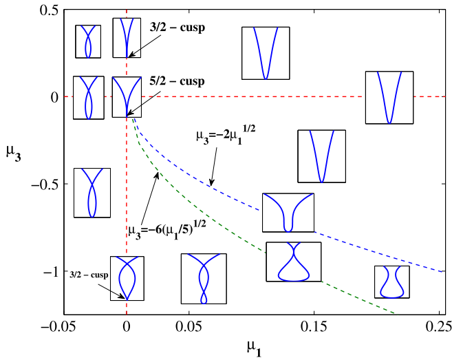
Fig. 6. Bifurcation diagram of the unfolding of the A_4 singularity (33). The bifurcation center \mu_1 = \mu_2 = 0 corresponds to a 5/2-cusp; for the critical case \mu_1 = 0 a 3/2-cusp singularity is formed at the tip, with the curve self-intersecting for \mu_3 > 0 . In the remaining four quadrants, for \mu_3 \propto |\mu_1|^{1/2} the curve forms a sequence of self-similar shapes. Along the line \mu_3 = -6\sqrt{\mu_1/5} , ( \mu_1 > 0 ), this sequence forms a single bubble, while for \mu_3 = -2\sqrt{\mu_1} , ( \mu_1 > 0 ), a channel with vertical tangents is formed. For \mu_3 < -6\sqrt{\mu_1/5} the curve has two double points, for \mu_1 < 0 a single double point.
