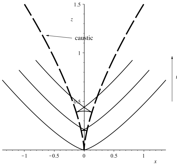
Fig. 15. The cusp catastrophe: wave fronts are swallowtails, the caustic is a cusp, as given by (74) and (75), respectively.
