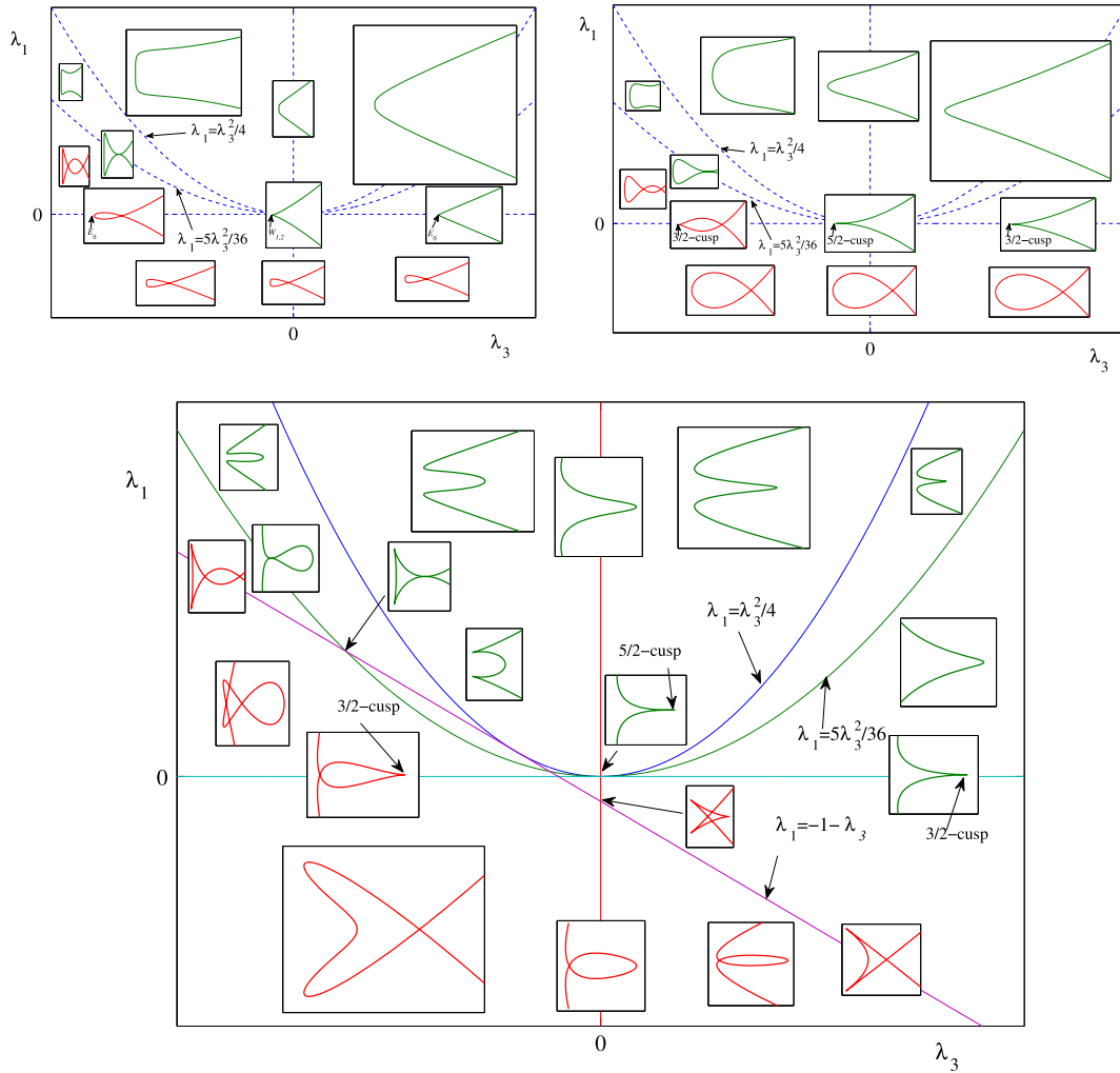
Fig. 12. Bifurcation curves for the W_{1,2} singularity with additional symmetry, see (47). On top, unfolding for s = 1 and s = 0 , at the bottom, the bifurcation diagram for s = -1 .
