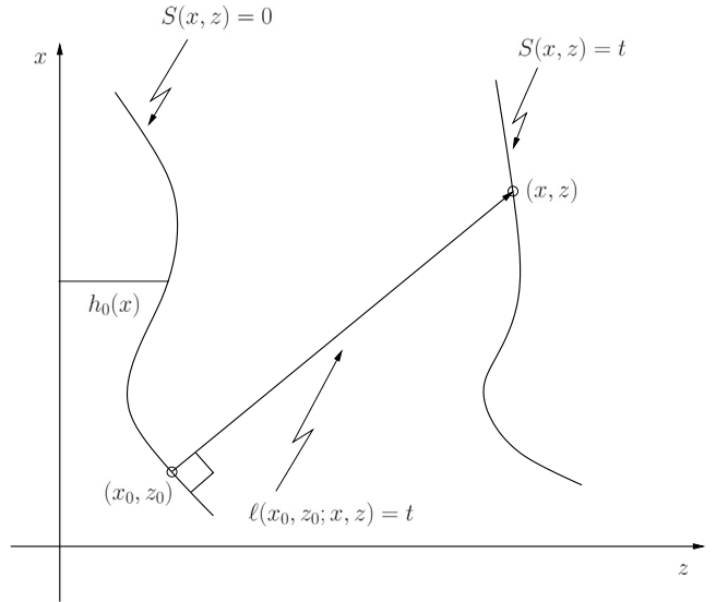
Fig. 14. A wavefront can be described either as the graph of a function z = h(x, t) , or as lines of constant value of the action S(x, z) . Rays are perpendicular to the wavefronts, and \ell(x_0, z_0; x, z) measures the optical path length between two points.
