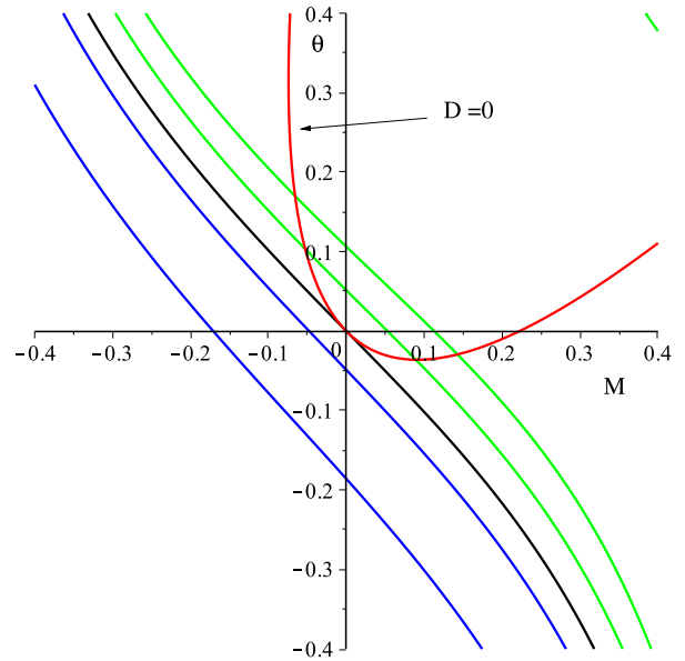
Fig. 18. The formation of a swallowtail. The solution front advances from left to right: blue (before the singularity), black (at the singularity), and green (after the singularity), when the front has two intersections with D = 0 . (For interpretation of the references to color in this figure legend, the reader is referred to the web version of this article.)
