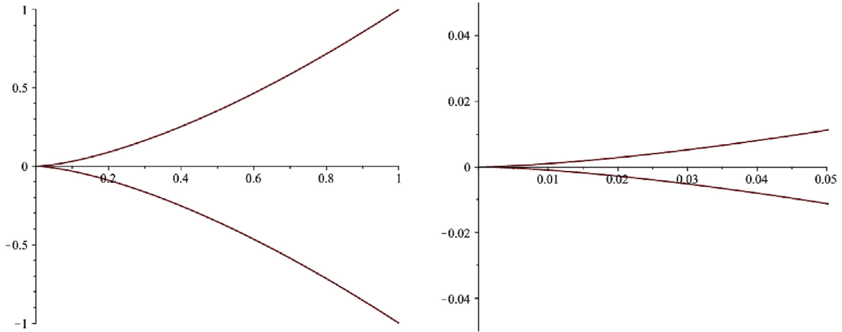
Fig. 5. The cusp (t^2, t^3) ; zooming into the tip, the cusp looks narrower, as seen on the right.
