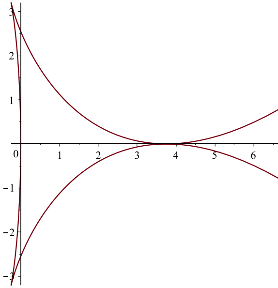
Fig. 11. A bubble in the form of a swallowtail, as described by the similarity function (46).
