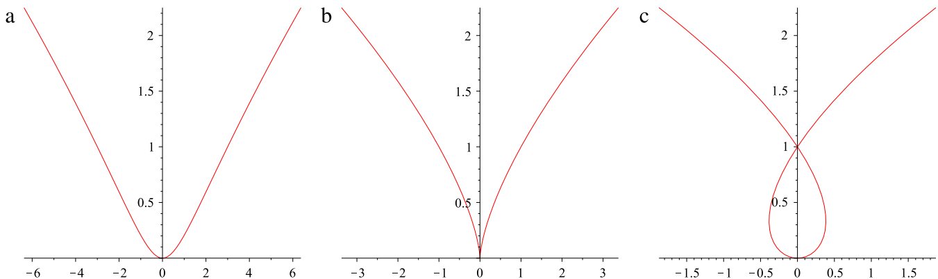
Fig. 7. The cusp similarity function (37) for s = 1, s = 0 , and s = -1 , from left to right.
