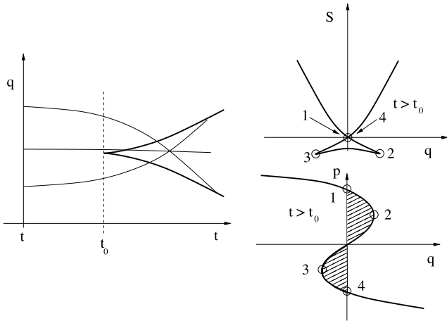
Fig. 13. The generic form of a cusp singularity. On the left, lines are trajectories with the caustic line shown in bold. Inside the caustic, three different trajectories correspond to any given point. On the right, the solution at a time t > t_0 after the singularity. The action has the form of a swallowtail, while the momentum forms an s-curve. Taking a path along which S is single-valued corresponds to jumping from the upper branch of the s-curve to the lower branch in such a way that the shaded areas are equal.
