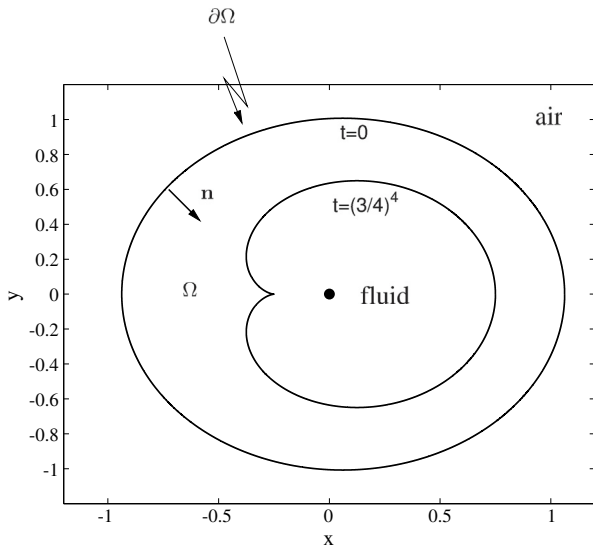
Fig. 19. The formation of a cusp in the Hele-Shaw problem with suction at the origin, using the exact solution (97) with coefficients (98). The initial condition is a_1(0) = 1, a_2(0) = 1/16 . A cusp is formed at t = (3/4)^4 .
