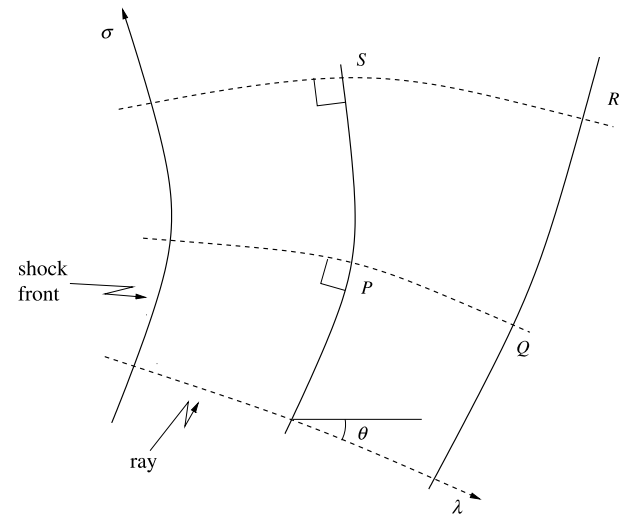
Fig. 17. The “geometrical optics” approximation of shock dynamics. Shock fronts and rays form an orthogonal plane coordinate system (\lambda, \sigma) ; \lambda measures the distance along rays, \sigma the distance along a shock front.
