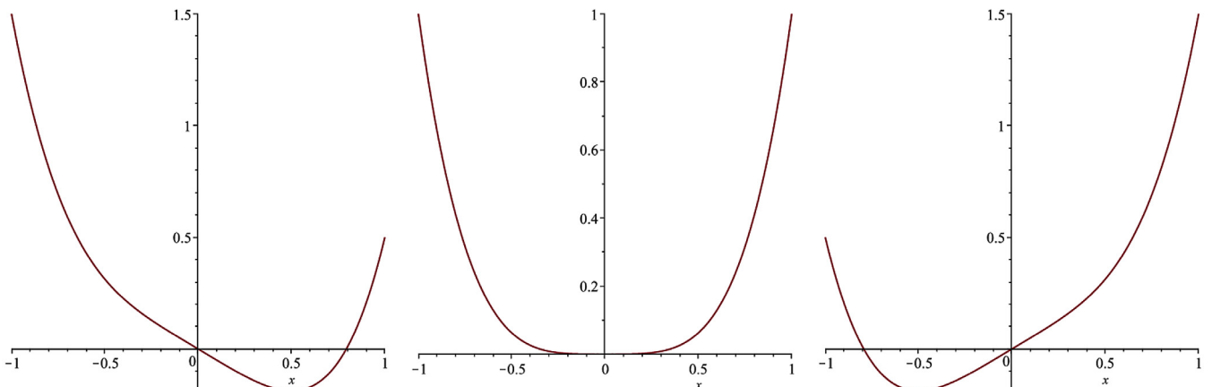
Fig. 3. The bifurcation of the A_3 catastrophe, illustrated for \epsilon_2 = 0 . When \epsilon_1 = 0 the minimum point at the origin is quartic, while for \epsilon_1 \neq 0 the order of the minimum becomes quadratic.
