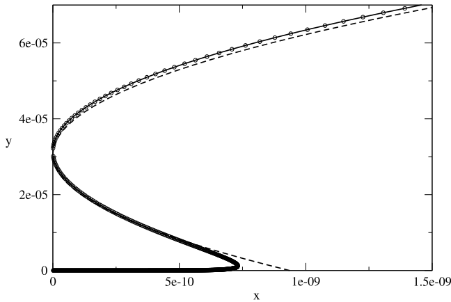
Fig. 23. The neighborhood of the bubble for k' = 10^{-2} . The solid line is the full solution (129), (130), with B adjusted such that pinch-off occurs (both sides of the profile touching). The symbols are the asymptotic result (135), with \delta determined by (137). The dashed line is the scaling function (139).
