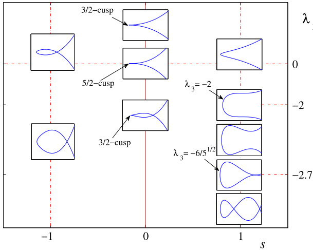
Fig. 8. The bifurcation diagram of the unfolding of A_4 singularity in its scaled form (38).
