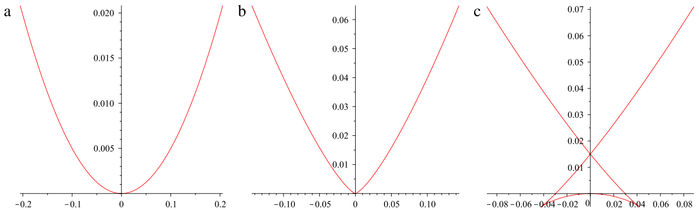
Fig. 10. The swallowtail similarity function (45) for s = 1 , s = 0 , and s = -1 , from left to right.
