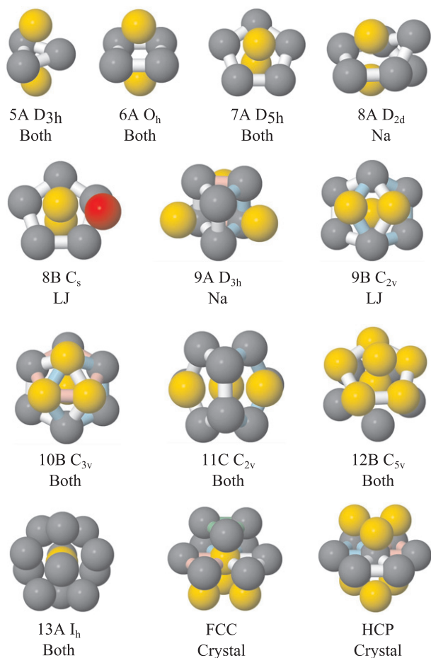
Figure 3. Structures of LJ and Na clusters, nomenclature following [31], and their point group symmetries. The colours denote the method used for cluster detection by the TCC algorithm: three-, four- and five-membered ring atoms are grey, spindle atoms are yellow, additional atoms to a basic cluster are red (here just 8B which is detected from 7A clusters), and rings are coloured white, blue, pink and green.
