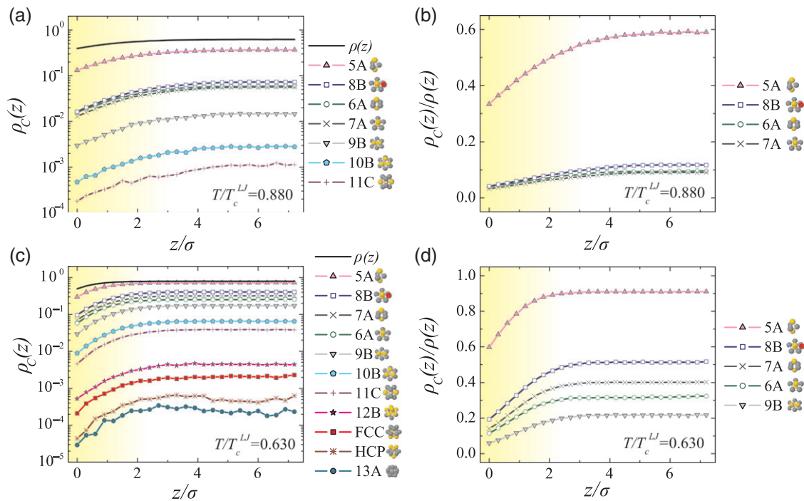
Figure 5. TCC analysis of the Lennard-Jones interface \rho_C(z) denotes the density of particles belonging to a particular cluster type. \rho(z) reproduces the data in Figure 4. (a) T=0.95 ( T/T_c^{LJ} = 0.880 ). (c) The triple point T_{tr}^{LJ} = 0.68 ( T/T_c^{LJ} = 0.630 ). (d) Same data as (c) but normalized by \rho(z) . Interface increases from z=0 , black interface density profile. Yellow shading is a guide to the eye, indicating the width of interfacial region.
