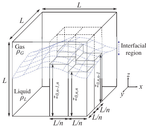
Figure 2. Identification of the position of a capillary perturbed interface. The interface is shown in blue and the cube is split into n^2 columns i, j . The interface is assumed flat in each column and the position is extracted by a fitting step function (Equation (4)) to the columnar density profile \rho_{i,j}(z) . Note periodic boundaries apply in the x and y directions only.
