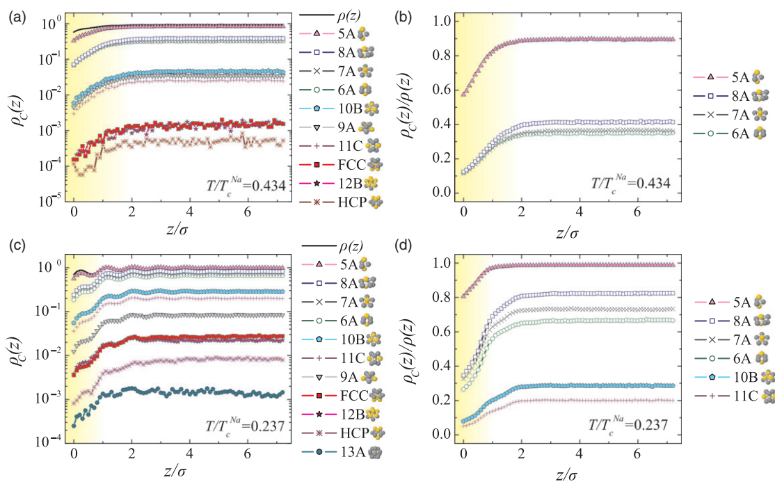
Figure 6. TCC analysis of the sodium interface \rho_C(z) denotes the density of particles belonging to a particular cluster type. \rho(z) reproduces the data in Figure 4. (a) T=0.542 ( T/T_c^{\text{Na}} = 0.434 ). (c) Near the triple point T_{\text{tr}}^{\text{Na}} = 0.297 ( T/T_c^{\text{Na}} = 0.237 ). (b) and (d) Same data as (a) and (c) but normalized by \rho(z) . Yellow shading is a guide to the eye and indicates the interfacial region.
