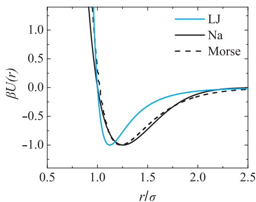
Figure 1. Model potentials used. Blue line, Lennard-Jones (LJ); solid black line, sodium (Na); dashed line, Morse potential with range parameter \rho_0 = 4.05 .
