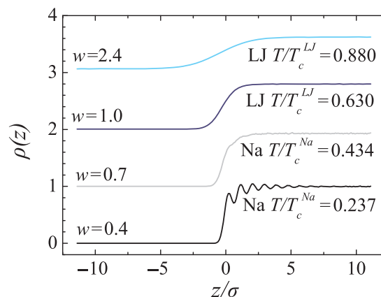
Figure 4. Interfacial profiles \rho(z) . From top, Lennard-Jones T = 0.95 , T = 0.68 , sodium T = 0.542 , T = 0.297 . Data offset for clarity. The sodium interface at the lowest temperature shows a very pronounced surface layering. The interfaces have all been centred at z = 0 .
