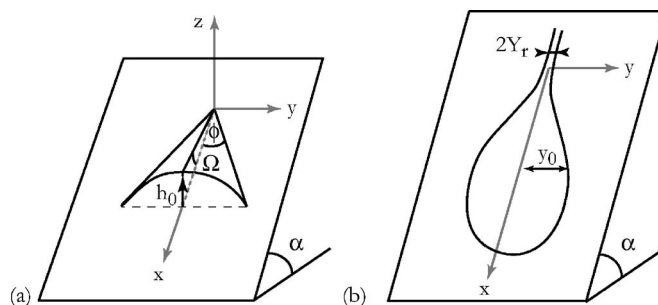
FIG. 2. Sketch of a the drop sliding down an inclined plane. On the left we show the local geometry of the corner, while on the right a rivulet of width 2Y_r has formed. The local width of the drop is y_0(x) , its thickness is at the centerline h_0(x) .
