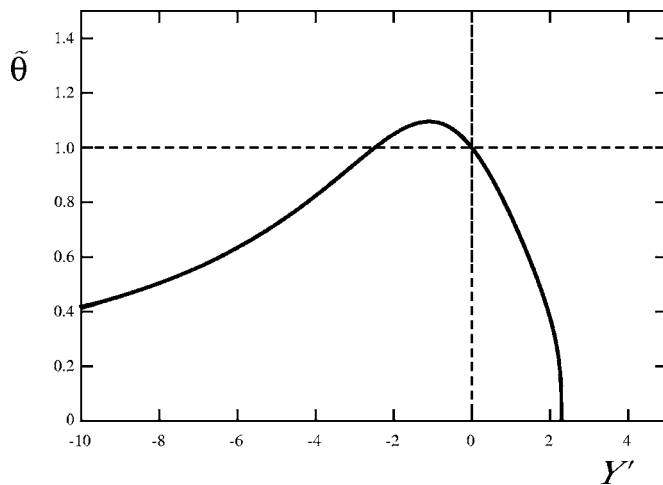
FIG. 10. The function \tilde{\theta}(Y') according to (27), plotted with \epsilon=1/\sqrt{10} and C=3/2C_{cr} . The maximum of this curve plays a crucial role in the selection of the drop solution (see text).
