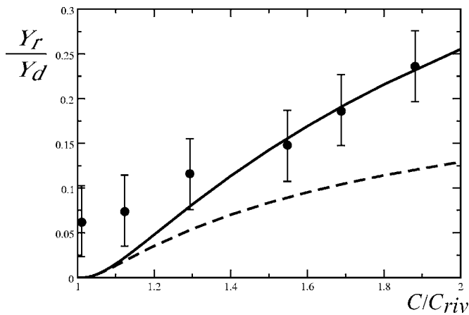
FIG. 9. The rivulet size Y_r (normalized by the maximum drop width Y_d ) as a function of C as obtained from numerical resolution of (36) ( \epsilon=0.344 , taken from experiment). Dots are experimental measurements. Close to the transition, the rivulet immediately starts to break up in a sinusoidal mode; in that case Y_r is taken as the average width. The dashed line corresponds to (38), with \bar{Y}=0.37 and a=1.0515 .
