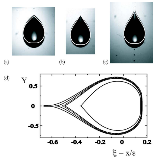
FIG. 6. (a–c) Same as in Fig. 5 compared to numerical simulation of Eq. (31). We fixed C/C_{riv} at the corresponding experimental values Ca/Ca_{riv} . The only adjustable parameter here is the length scale of the numerical curves. The experimental profiles systematically have a larger aspect ratio due to contact angle hysteresis. (d) Dimensionless drop profiles obtained from Eq. (31) for various C . The dashed curve corresponds to C_{riv} .
