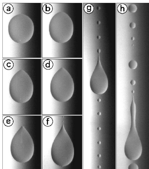
FIG. 1. Drops of silicone oil sliding down planes at increasing inclination angle (Ref. 5). As the velocity increases, a corner first forms, which becomes unstable to the ejection of drops at even higher speeds.
