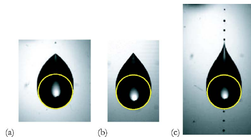
FIG. 5. Drops of viscosity 104 cP at different regimes: (a) corner, (b) cusp, and (c) rivulet. The corresponding values of Ca/Ca_{riv} are 0.761, 0.975, and 1.047, respectively. In all cases the front of the drop is fitted extremely well by a circle.
