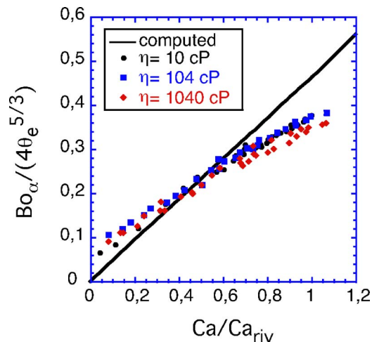
FIG. 7. The rescaled Bond number as a function of C . As predicted by (35), the experiment for different viscosities collapse onto a universal curve. To compute the theoretical curve, we chose a typical value of \epsilon=1/\sqrt{10} . Theory somewhat overestimates the slope and does not display the offset at Ca=0 due to contact angle hysteresis.
