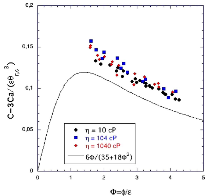
FIG. 3. The normalized speed C of the drop as a function of the normalized opening angle \Phi . Symbols represent rescaled experimental data for three different viscosities (see Table I). The data were rescaled using the receding static contact angle \theta_r .
