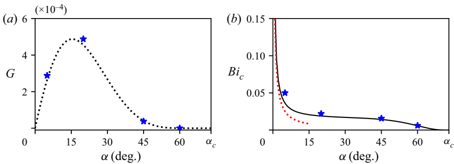
Figure 6. ( a ) Torque, G , acting on the vertical radius of the semi-circle considered in § 4.1 using the corresponding Moffatt solution (dotted) and from the viscoplastic numerical simulations shown in the top row of figure 5 (stars), as a function of the wedge half-angle, \alpha . ( b ) The corresponding critical Bingham number, Bi_c , calculated from (4.2) (solid line), as a function of the wedge half-angle, \alpha . The red dotted line shows the divergent behaviour as \alpha \rightarrow 0 , given by Bi_c \sim 0.0022/\alpha , while the stars indicate the smallest Bingham numbers of numerical simulations in which the new eddy has not yet opened up (and, hence, represent numerical upper bounds for Bi_c ).
