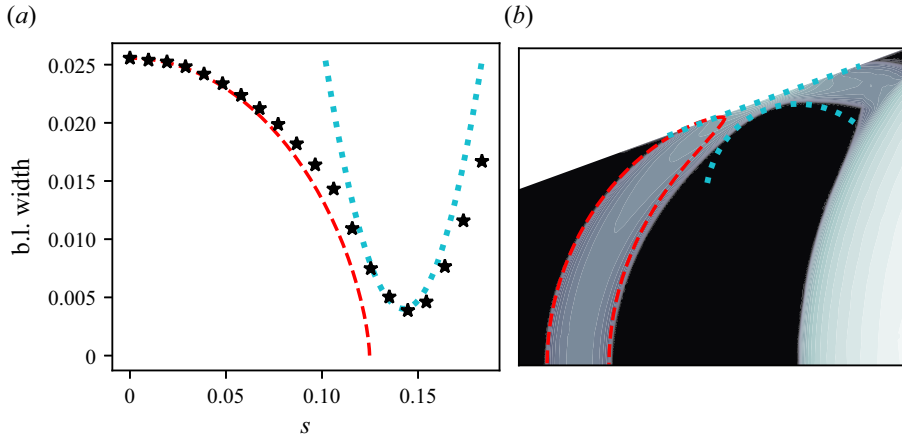
Figure 9. (a) Boundary layer width as a function of streamwise coordinate, s , from the numerical solution for \alpha = 20^\circ and Bi = 0.02 (black stars) and the asymptotic solutions (4.24a,b) (cyan dotted) and (4.33) (red dashed). (b) A contour plot of log strain rate from the same numerical simulation (black regions represent unyielded plugs) and the predicted boundaries of the shear layer from these asymptotic solutions (colours correspond to left panel).
