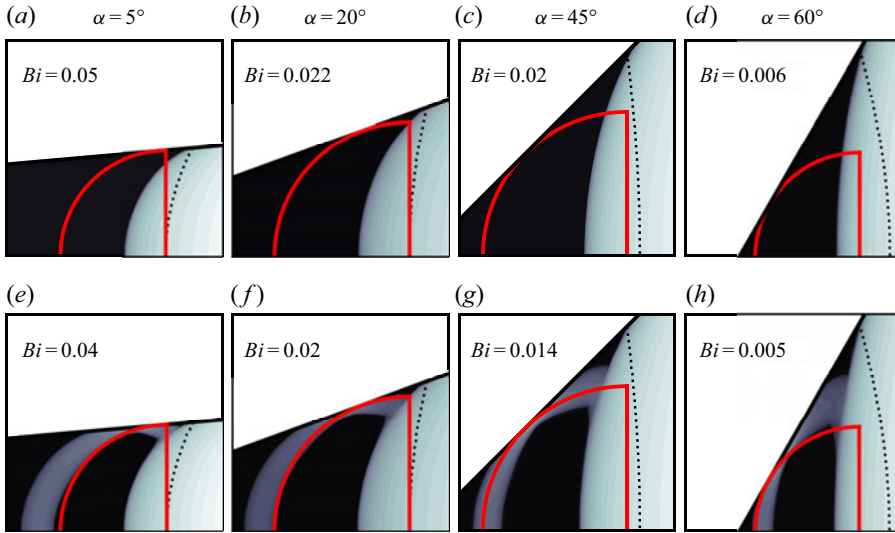
Figure 5. Examples of solutions before ( a–d ) and after ( e–h ) a new eddy has formed. The dotted line shows the dividing streamline \psi_V = 0 from the corresponding Moffatt solutions while the red lines show the semi-circles considered in § 4.1.
