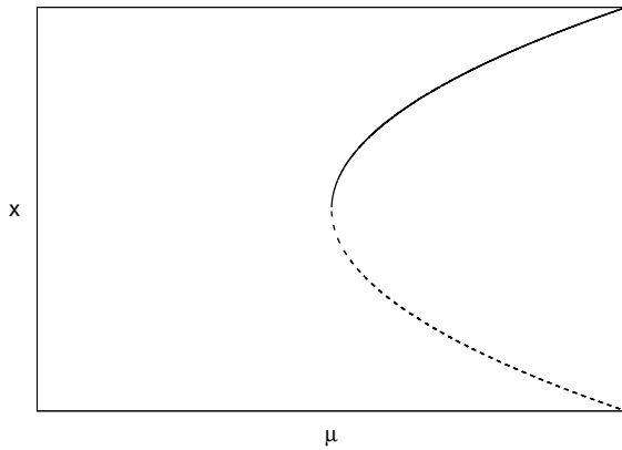
Figure 6: The fold bifurcation. Here, and in the later figures, solid lines indicate stable fixed points and dotted lines unstable fixed points.
