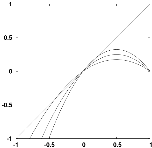
Figure 10: The logistic map \Phi_r for r = 0.7, 1, 1.3 illustrating the transcritical bifurcation.
