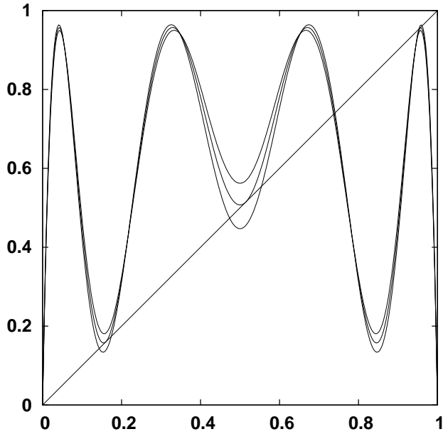
Figure 12: The map \Phi_r^3 for r = 3.8, 1 + \sqrt{8}, 3.856 illustrating the birth of a stable and unstable pair of period three orbits in a fold bifurcation.
