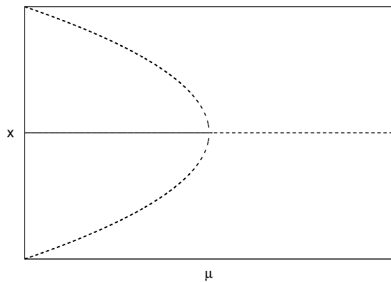
Figure 9: The subcritical pitchfork bifurcation (or period doubling, or Hopf, as in Fig. 8).
