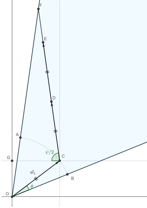
FIGURE 6. Diagram of \mathcal{A}_1 in case (C3)
