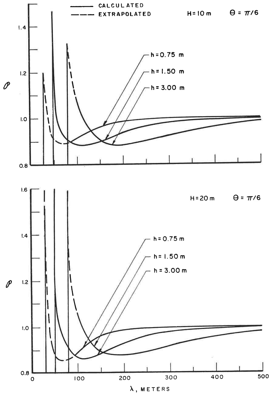
FIG. 13. BOTTOM PRESSURE FLUCTUATION \rho VERSUS INCIDENT WAVE LENGTH \lambda
