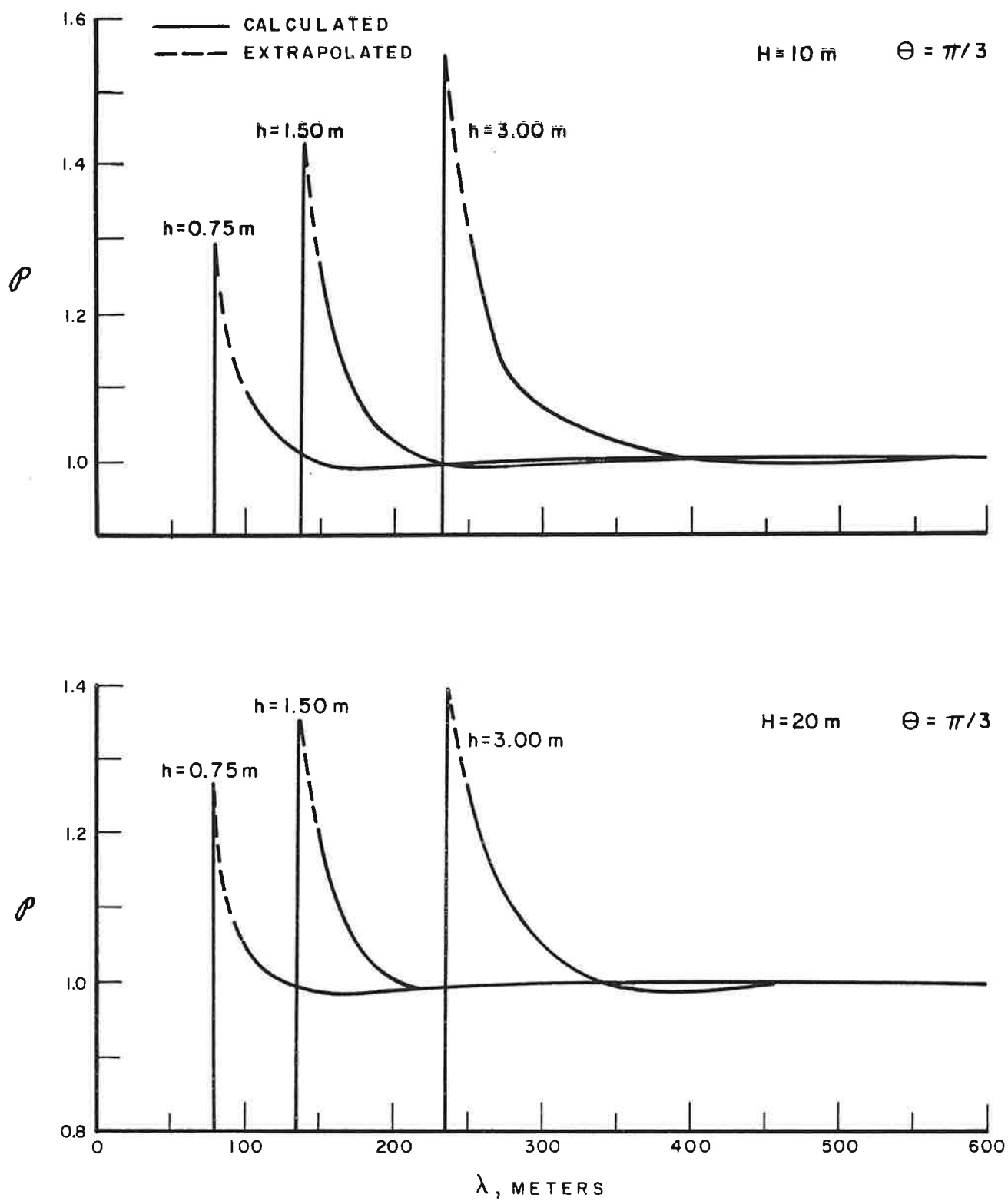
FIG. 15. BOTTOM PRESSURE FLUCTUATION \rho VERSUS INCIDENT WAVE LENGTH \lambda
