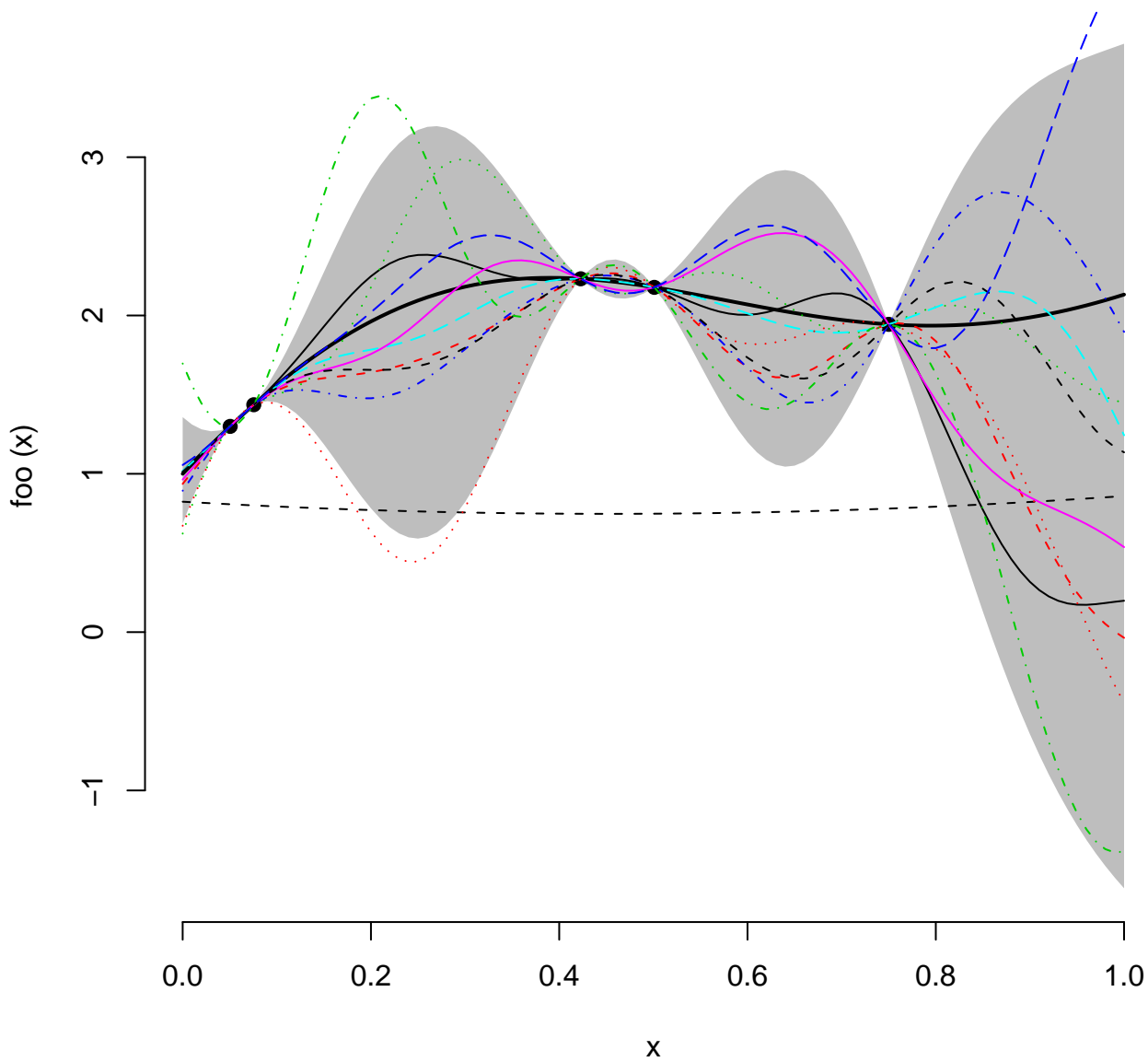
Function with evaluations, \pm 2 sd prediction, and regression line
