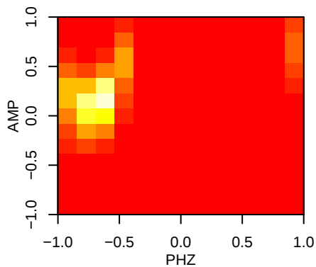
PHZ (periodic)
