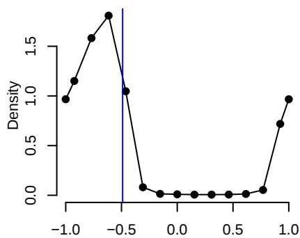
PHZ (periodic)
