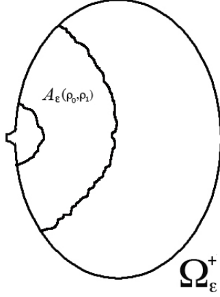
FIGURE 10. The annulus where the convergence is uniform.
