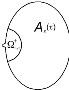
FIGURE 8. The sets \Omega_{\varepsilon, \tau}^+ and A_\varepsilon(\tau) .
