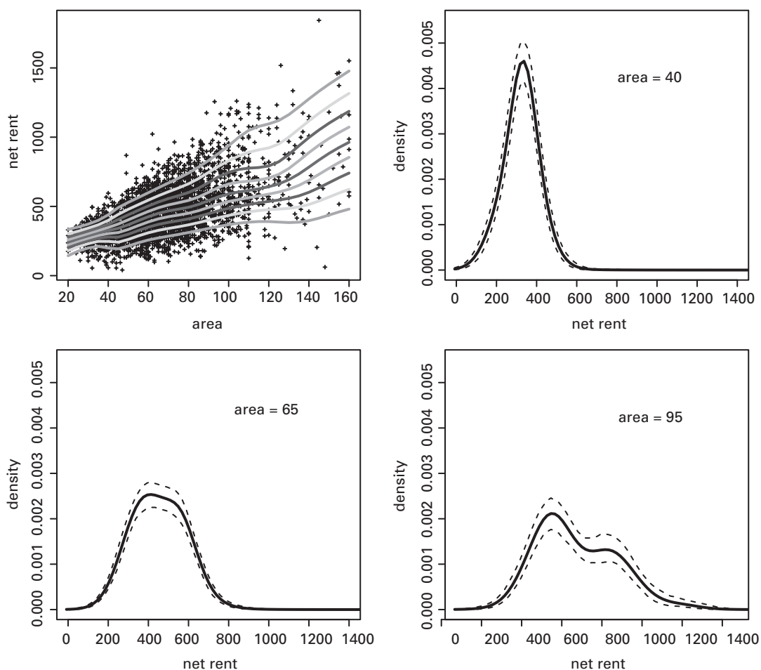
Figure 1 Munich rental guide data: a simple model fit using DPdensity. Top left: raw data, net rent vs area, with 10%, 20%, ..., 90% decile curves computed from the posterior mean of the cumulative conditional distribution of rent given area. Other panels: fitted conditional densities for rent, given area = 40, 65 and 95, respectively, with 90% credibility bands
